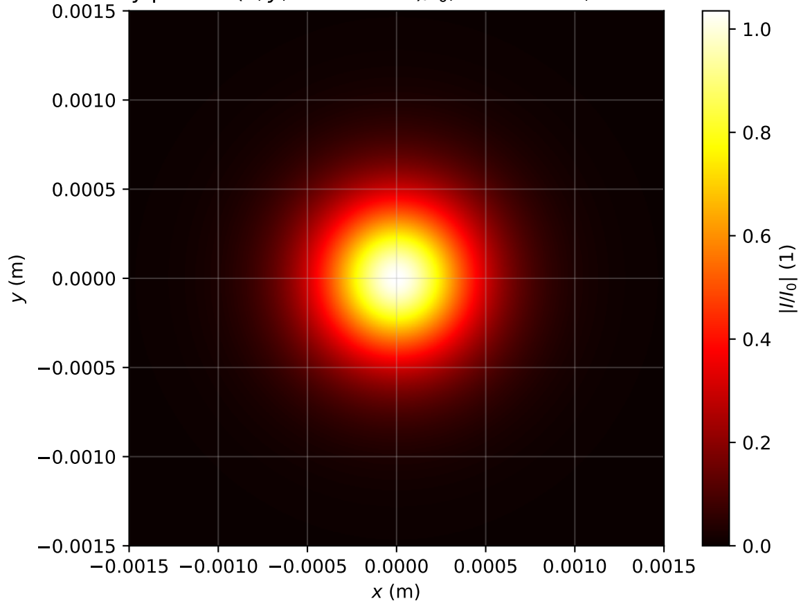
Intensity profile I(x, y, z = 3.264m)/I_0 , \text{Pin}=0.8\text{Pcr} , artificial time
